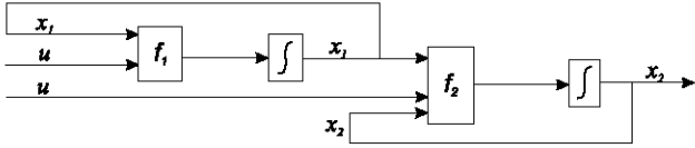
Fig. 1. Cascaded subsystems.
